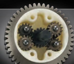
Planetary Differential
